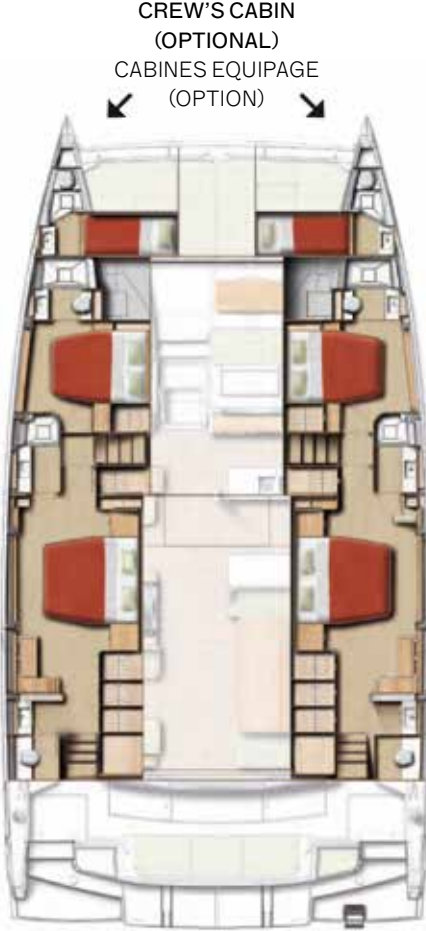
4 DOUBLE CABINS / 4 BATHS VERSION Version 4 cabines doubles / 4 sdb
